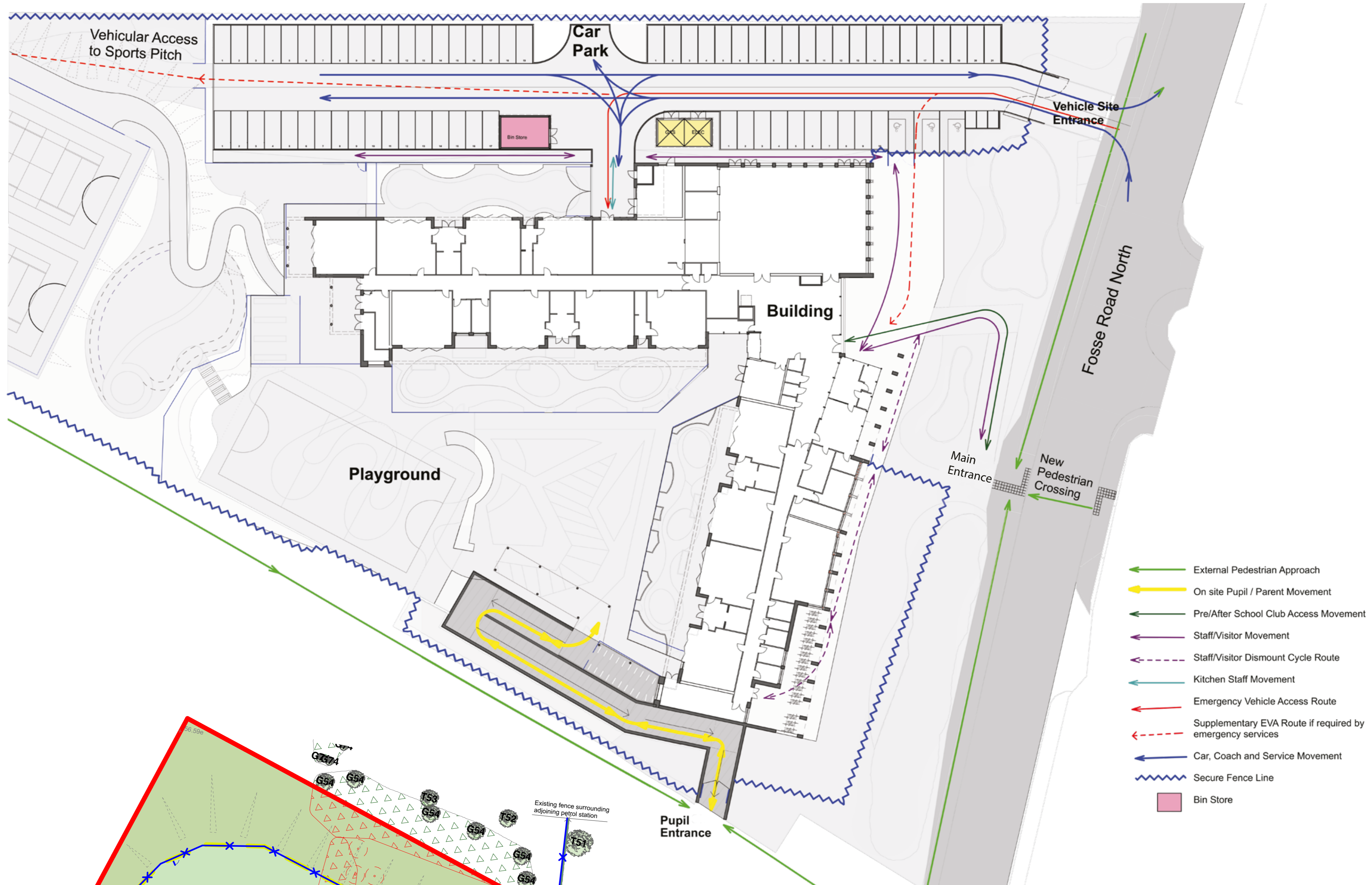
SITE CIRCULATION AND ACCESS PLAN
